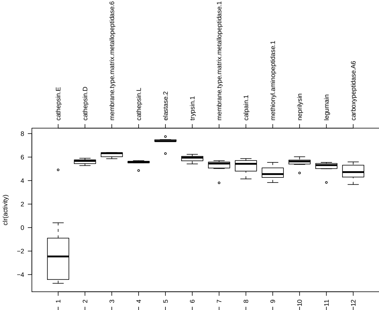
A (real data)
