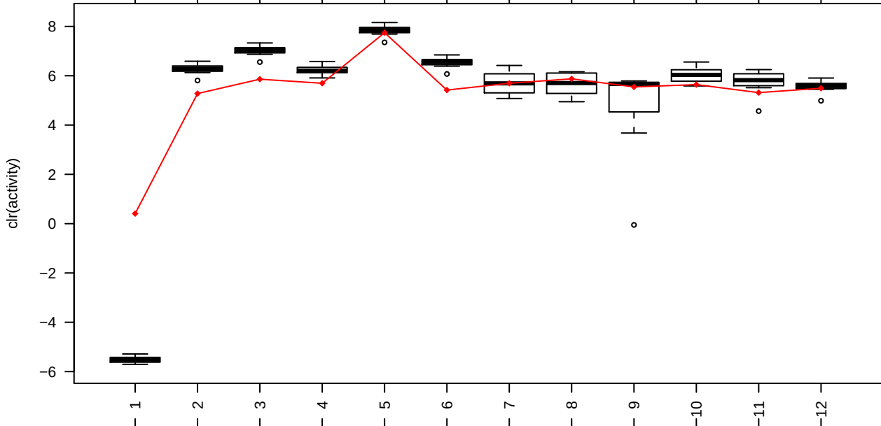
C (synthetic data with std = 0.01)
