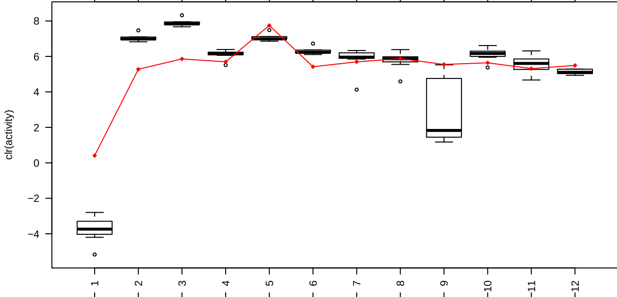
B (synthetic data with std = 0.1)
