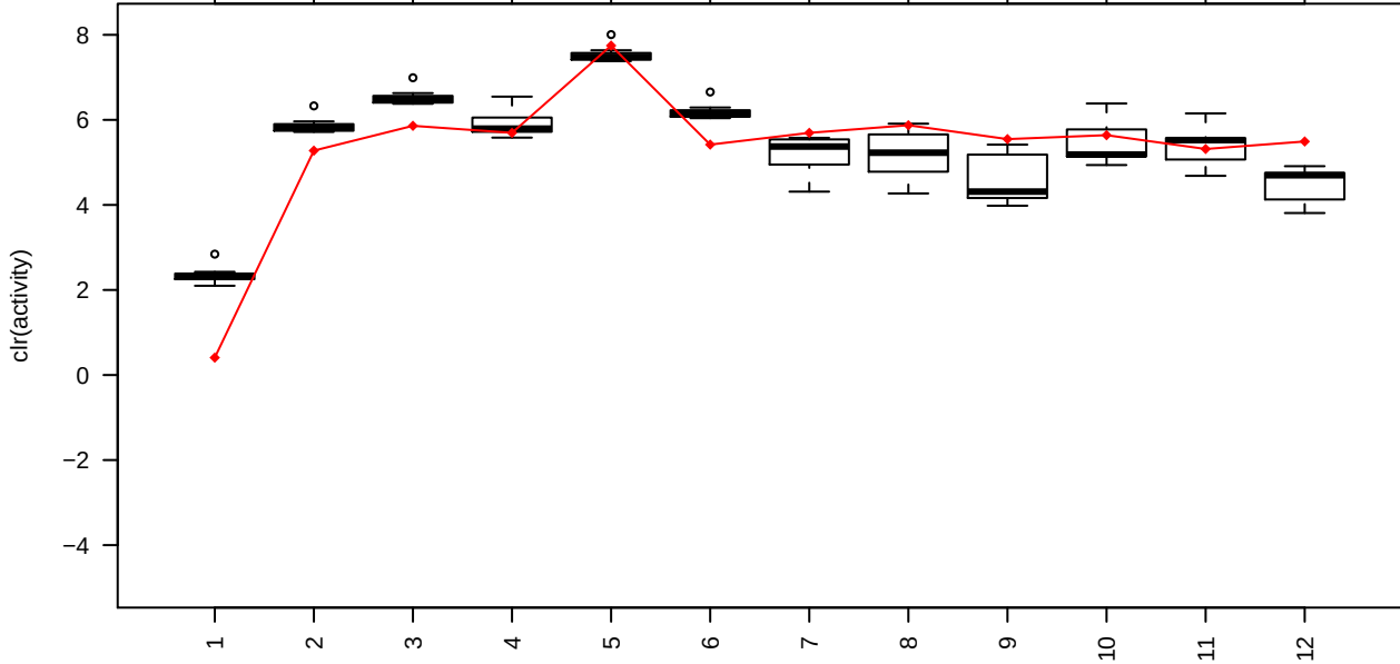
D (synthetic data with std = 0.001)
