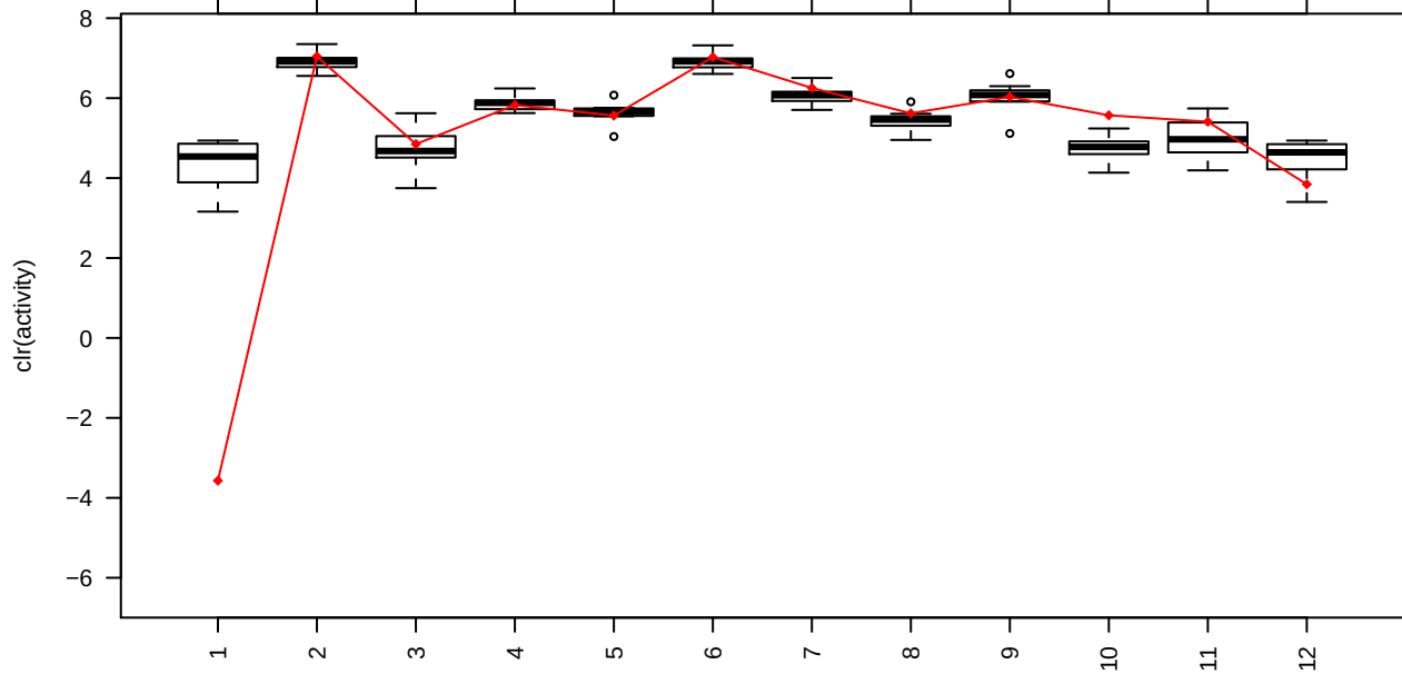
D (synthetic data with std = 0.001)
