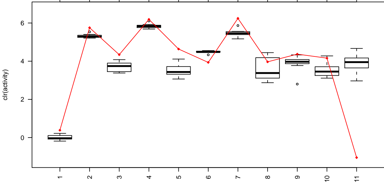
D (synthetic data with std = 0.0001)
